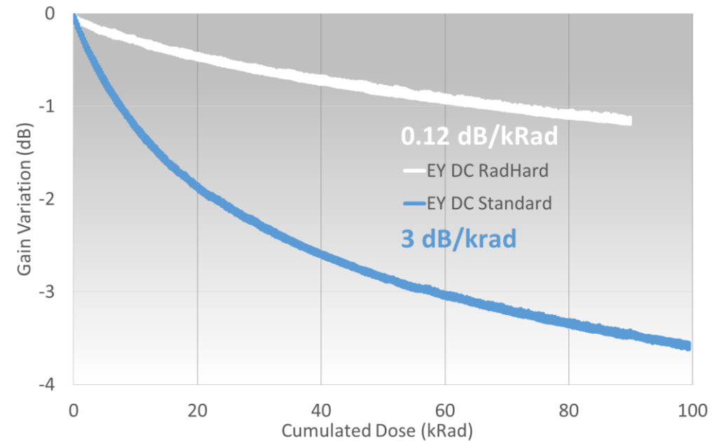
Single mode erbium/ytterbium doped Fiber Radiation Induced Attenuation Gain Variation (6μm core)
