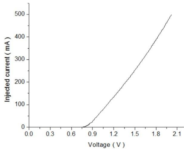
Laser I-V
