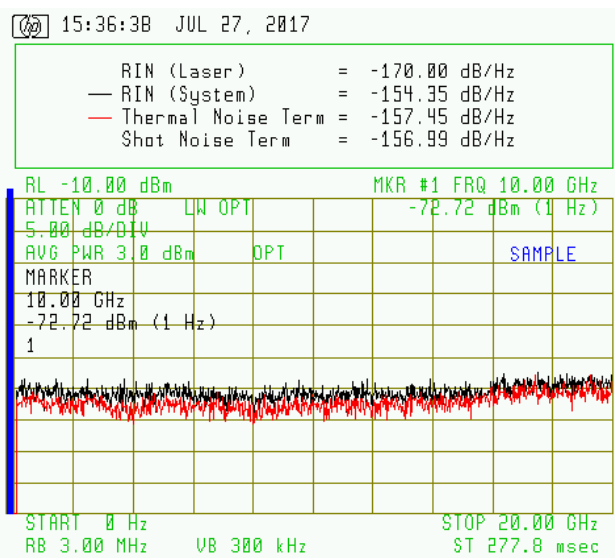
Laser RIN
